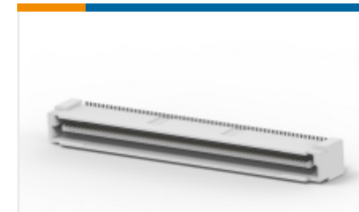
TE 系列/零件编号 3-5177986-5 0.8FH,P08H.5,120,08/Sn,TR,SC
