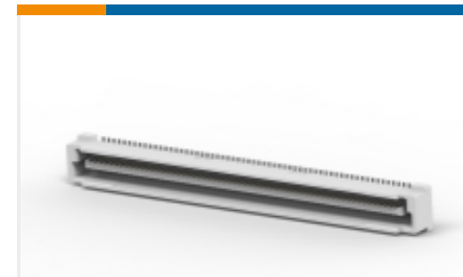
TE 系列/零件编号 5177986-5 0.8FH,P05H.5,120,08/Sn,TR,SC
