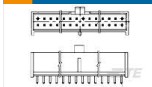
TE 系列/零件编号5-1658549-3 FPH-6022G=FLXPAC HDR P ST LF
