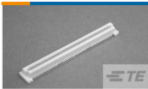
TE 系列/零件编号6123000-4 0.8FH,R05H.5,100,30/Sn,TU
