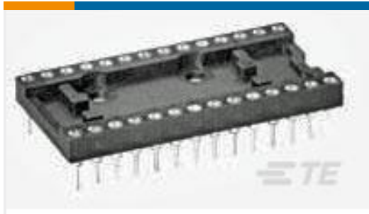
TE 系列/零件编号4-1437531-0 516-AG10D-ESL=500 SERIES SOCKET
