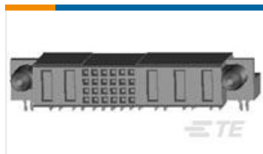
TE 系列/零件编号3-6450170-0 MBXL R/A RCPT 3ACP+24S+2P
