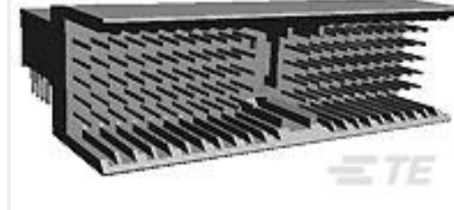
TE 系列/零件编号352131-1 Z-PACK/B RAMH.110P.
