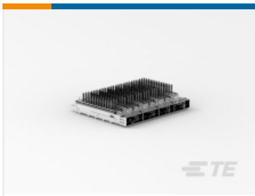
TE 系列/零件编号2170747-3 CAGE ASSY, 1X4, QSFP28, SPRING, HS, LP
