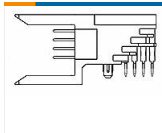
TE 系列/零件编号5223514-1 2MM FB,IS,ASY,024,SIG, HDR,SL
