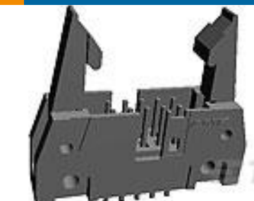
TE 系列/零件编号5746443-1 A/L UNIV HDR 10P ACT PIN LG LAT
