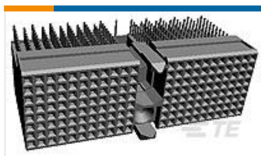
TE 系列/零件编号5646442-1 2MM HM,ASY,T-D,REC, TWIST TULIP
