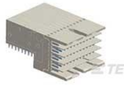
TE 系列/零件编号2042162-2 Right Angle Male Connector
