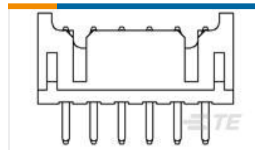
TE 系列/零件编号1470109-6 2.0mm Pitch Header,Dip 6p
