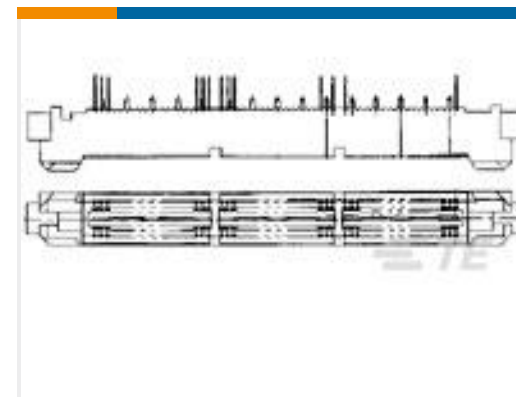
TE 系列/零件编号5767032-4 MICT, 788PLUG, 152, ASSY, 025, REC
