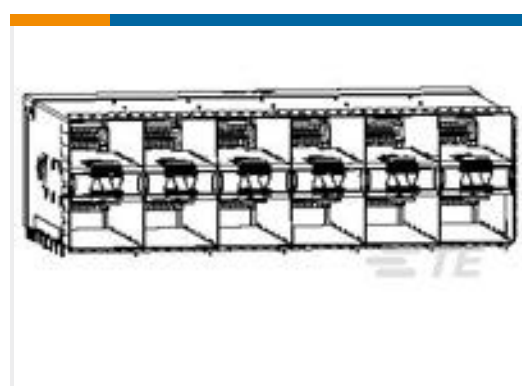
TE 系列/零件编号2198339-7 zSFP+ STACKED 2X6 RECEPTACLE ASSEMBLY
