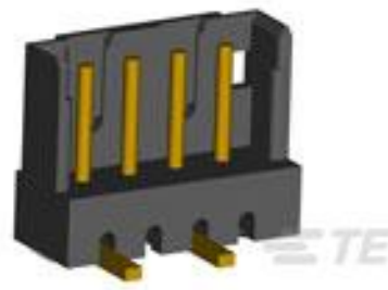
TE 系列/零件编号2106056-8 Assembly, Right Angle SMT Header, 4-Posi
