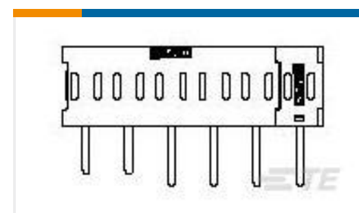
TE 系列/零件编号6766496-1 CONNECTOR, PIN, RIGHT ANGLE, SOLDER, FLAT
