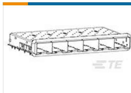
TE 系列/零件编号2198724-1 CAGEASSY,PRESSFIT,1X6, zSFP+
