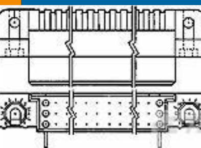
TE 系列/零件编号5746443-3 A/L UNIV HDR 16P ACT PIN LG LAT
