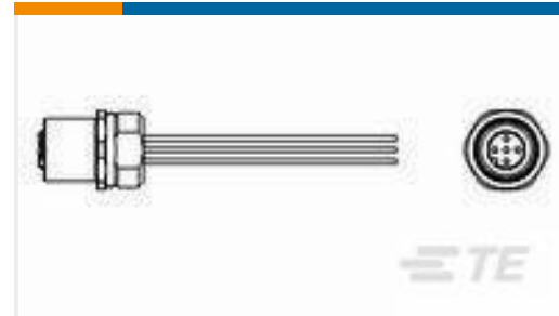
TE 系列/零件编号2273055-1 M12 Female pnl Mld Rear Mt PG9 pigt A
