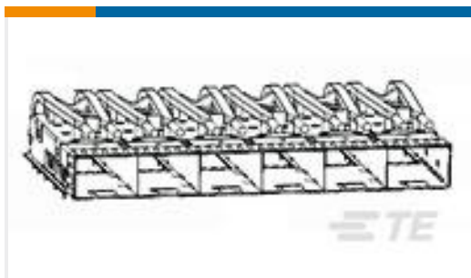
TE 系列/零件编号2227732-1 zSFP+ 1x6 Cage Assembly, Press-Fit
