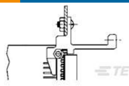
TE 系列/零件编号1-1977745-8 RCPT, 2.0MM, 38P,VRT MT, Sn
