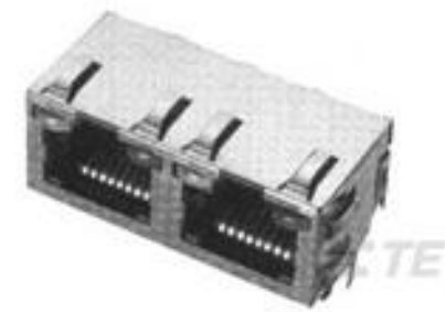
TE 系列/零件编号2- 6116353-4 INV MJ,1X2,PNL GRD,LED (G/G).120ST
