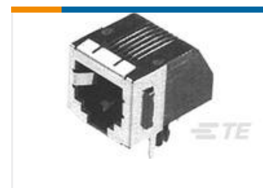
TE 系列/零件编号5558178-1 MJ,R/A,SMT,8P,PCB GRD, PNL STOP
