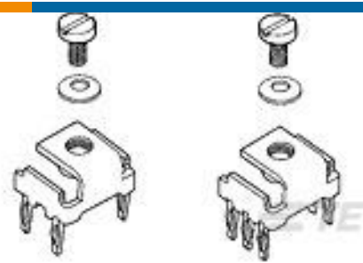
TE 系列/零件编号5213816-1 6P POWER TAP ASSY W /M4 SCREW
