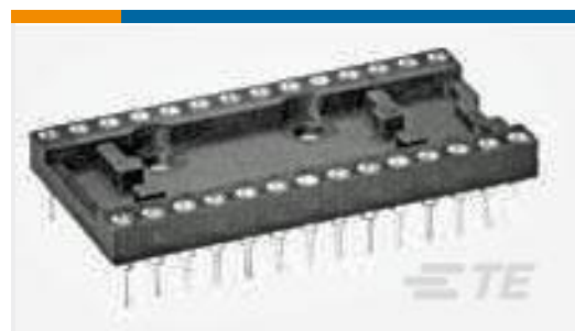
TE 系列/零件编号1-1571550-0 532-AG12D-LF=500 DIP, PCB,SN/SN
