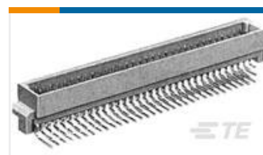
TE 系列/零件编号5536475-1 ASSY,PIN,EUROCARD, TYPE C,LEAD-FREE,96 PO LF
