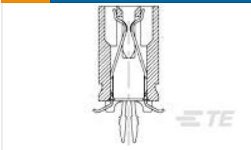
TE 系列/零件编号1-178316-3 DYNAMIC 3100 HDR ASSY 6P V K/X
