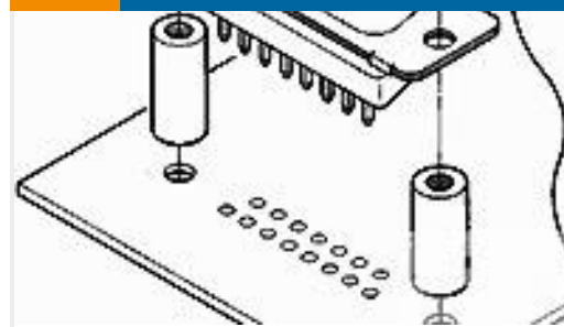
TE 系列/零件编号5205933-3 BUSHING KIT
