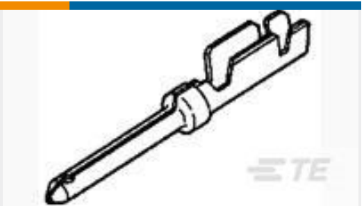
TE 系列/零件编号1658670-2 PIN CONTACT,22-28 AWG, 22 DF, AMPLIMITE
