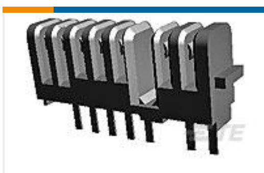
TE 系列/零件编号1747786-1 PACKING, REC. ASSY. 8POS. 2MM PITCH BATTE
