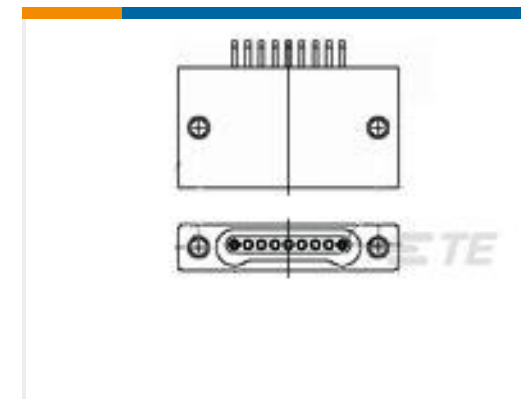
TE 系列/零件编号4- 1589462-4 SSM051L2HN = SMT CONN
