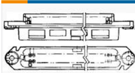
TE 系列/零件编号552303-1 ASSY, PLUG, 64 POS, C SLOT
