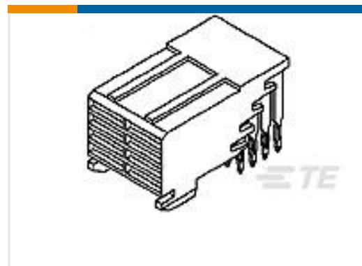
TE 系列/零件编号5536613-1 2MM FB,ASY,008,PWR, REC,SL,3.53
