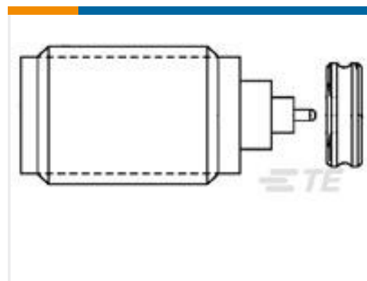
TE 系列/零件编号1053254-1 2058 5278 00 SMA FEEDTHRU JACK, SEALED
