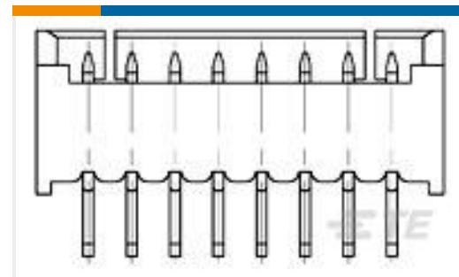
TE 零件编号2-1734598-9 1.25 WTB HDR DIP, L=2.3, 9P
