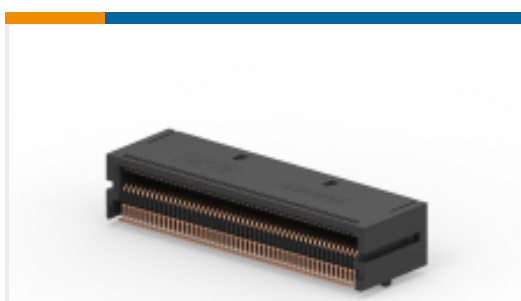
TE 零件编号2274845-1 CFP2 RECEPTACLE ASSEMBLY
