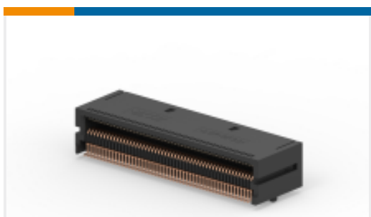
TE 零件编号2274845-1 CFP2 RECEPTACLE ASSEMBLY
