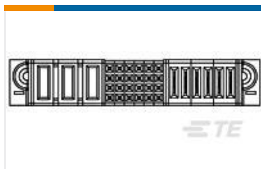
TE 零件编号6450860-7 MBXLE VERT RCPT 4P+28S+3ACP
