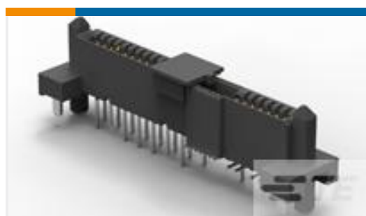
TE 零件编号1-1735104-3 SAS BACKPLANE RECEPT, VERTICAL
