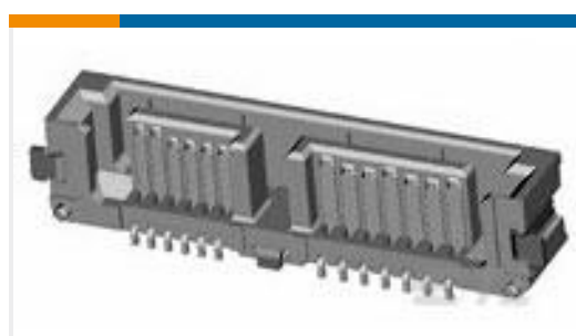
TE 零件编号1735574-3 Assembly Slimline SATA Plug Vertical, TH
