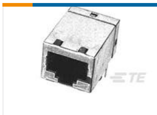
TE 零件编号1734795-4 RJ45,8P8C,SHD,W/O LED, DIP 50u"
